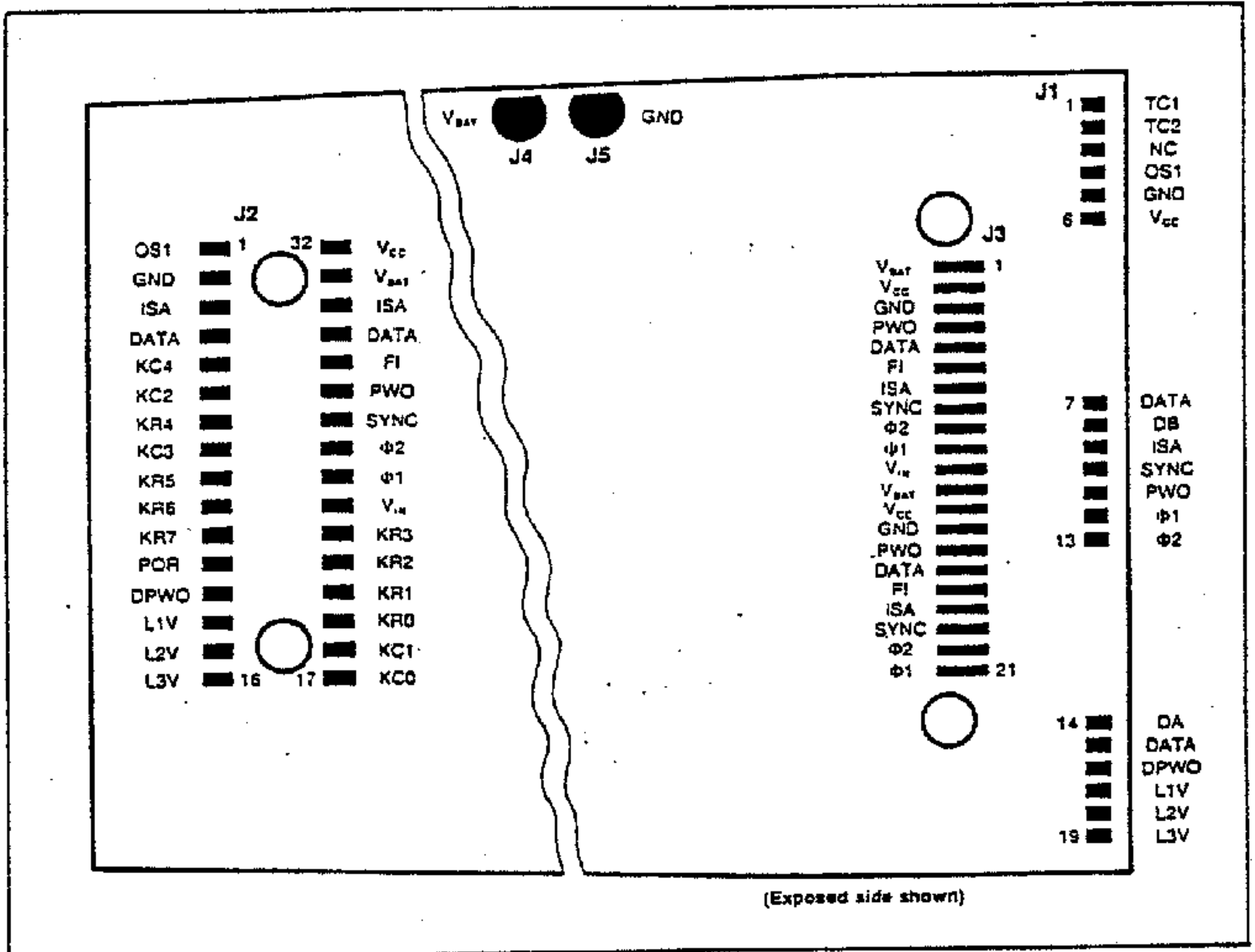
Figure 4-4. Contacts on Keyboard PC Board
