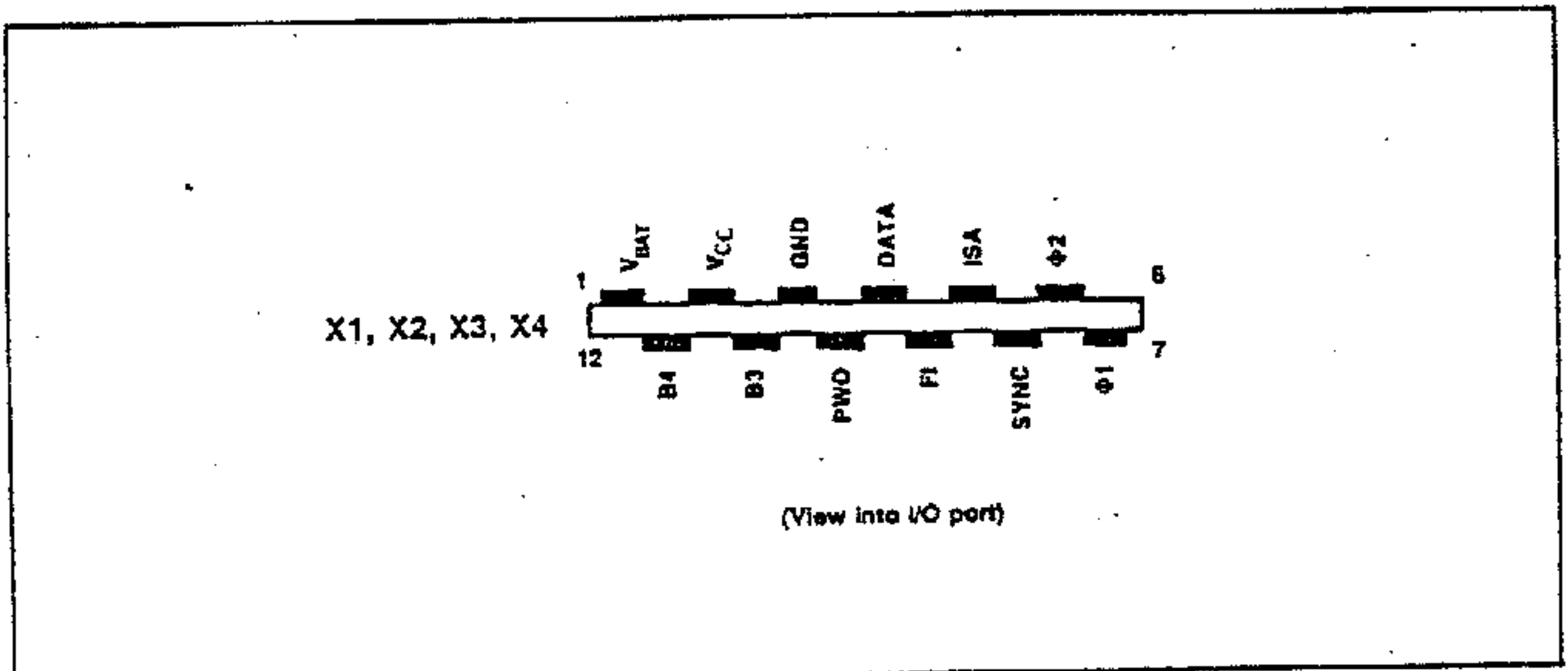
Figure 4-5. Contacts at I/O Port
