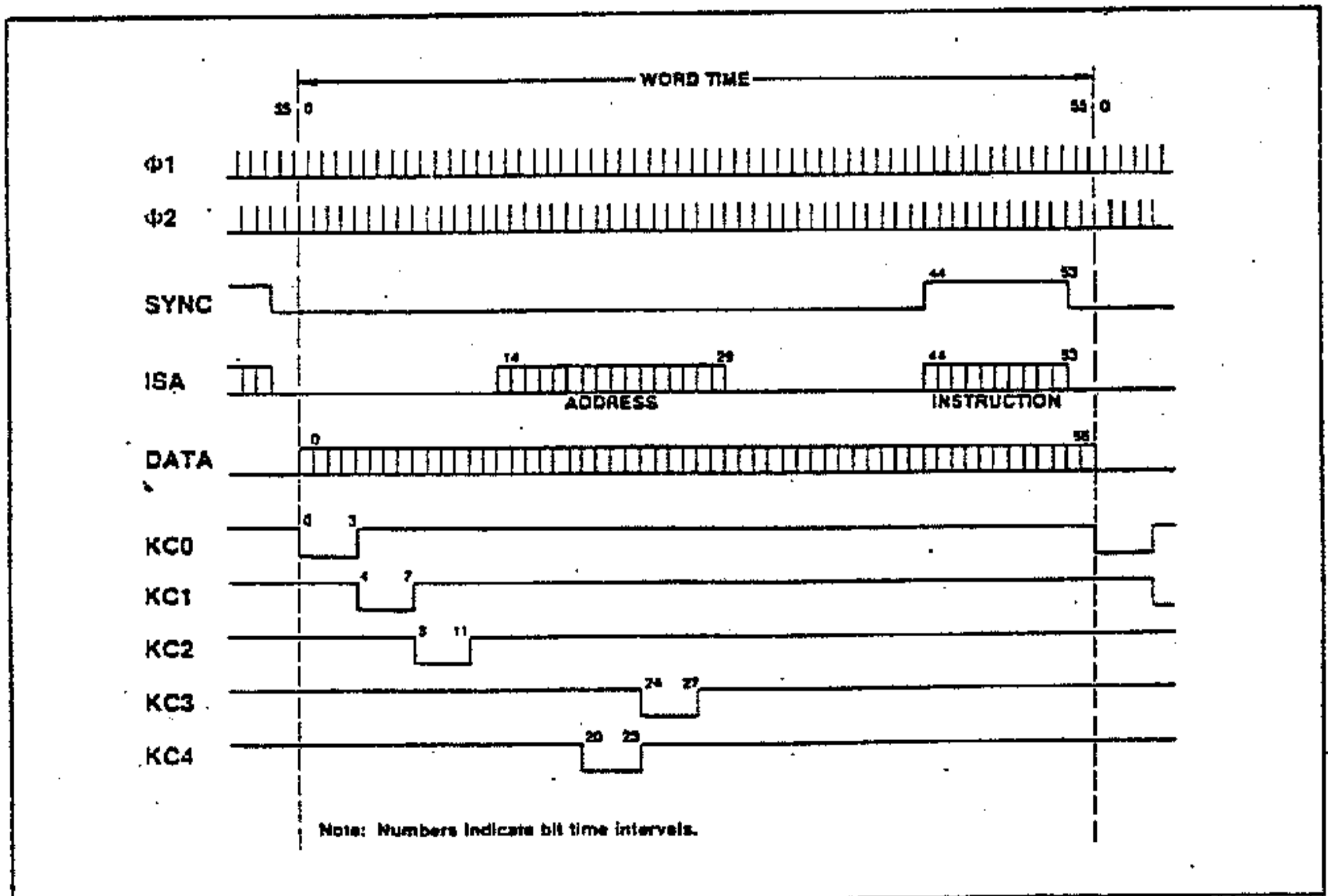
Figure 2-3. System Timing
