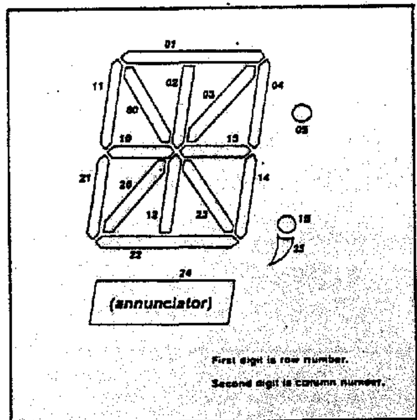
Figure 2-2. Display Character Structure
