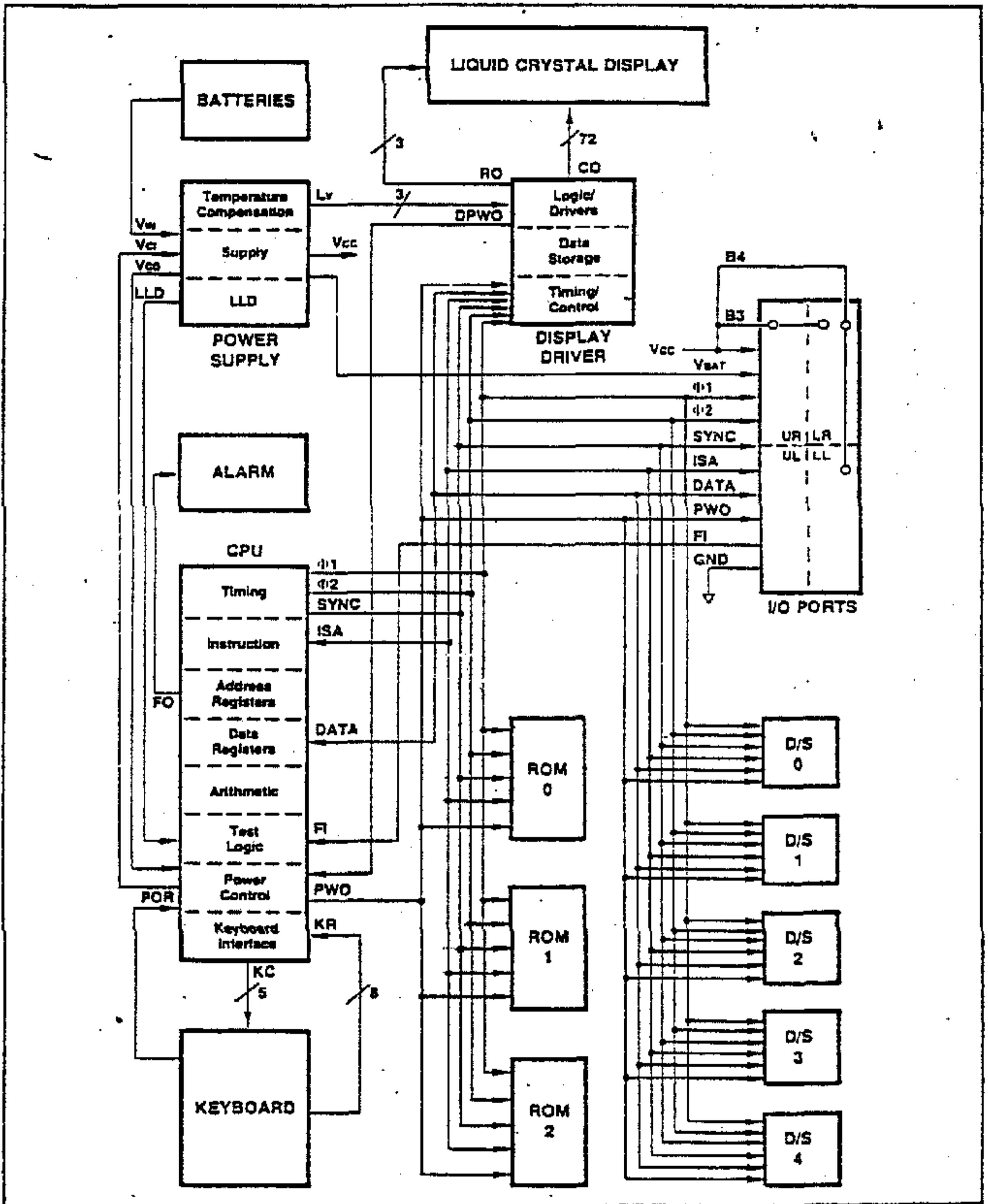
Figure 2-1. HP-41C Block Diagram
