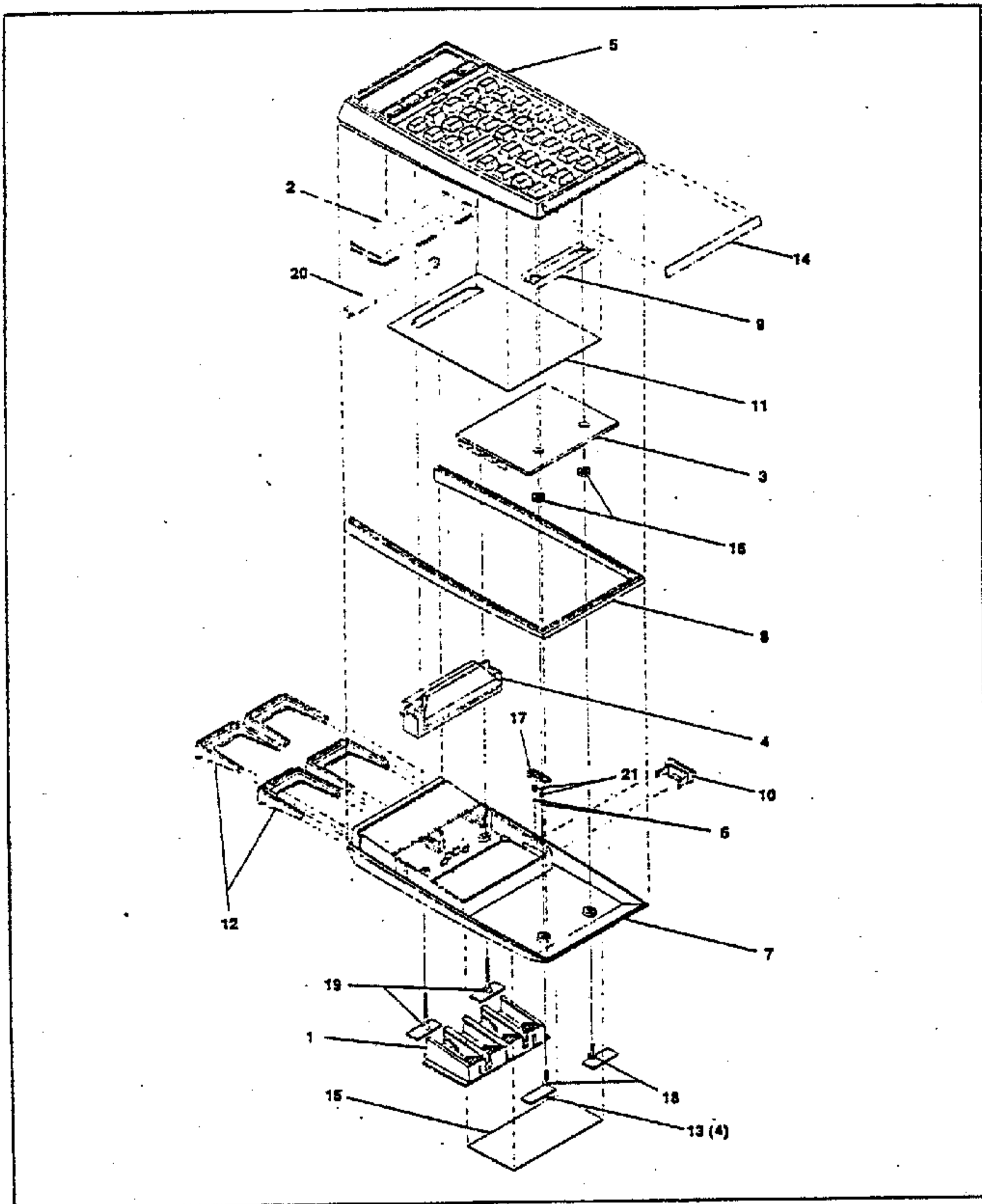
Figure 6-1. HP-41C Exploded View
